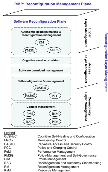
Fig. 3: The Reconfiguration Management Plane Model for Autonomously Reconfigurable Elements.
