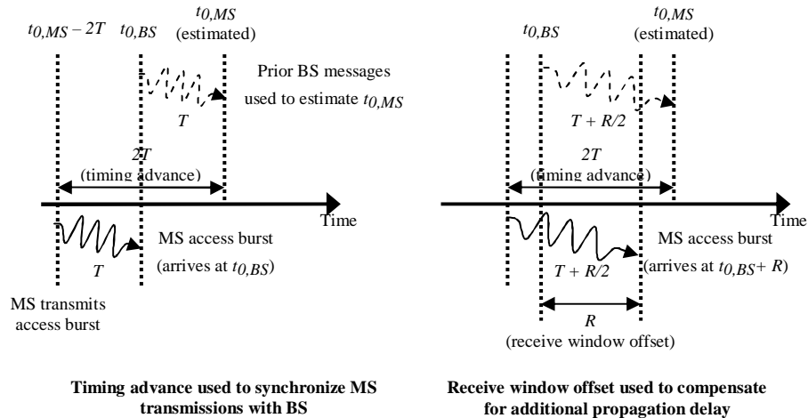
Figure 2: Use of Timing Advance and Receive Window Offset in GSM
