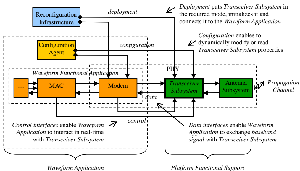
Figure 3: Transceiver Subsystem and related capabilities
